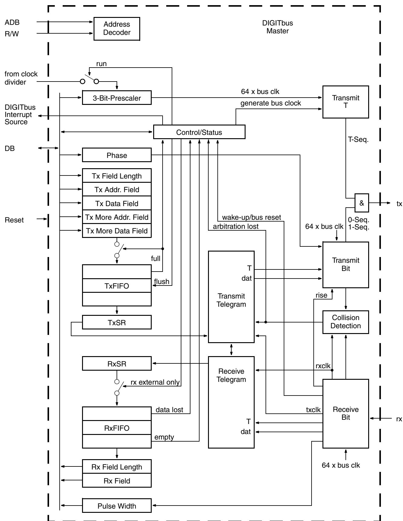
Fig. 23-2: Block Diagram
