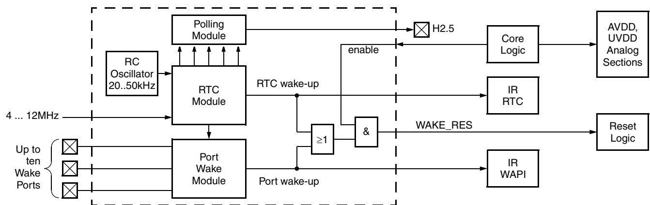
Fig. 8–1: Power-Saving Module
