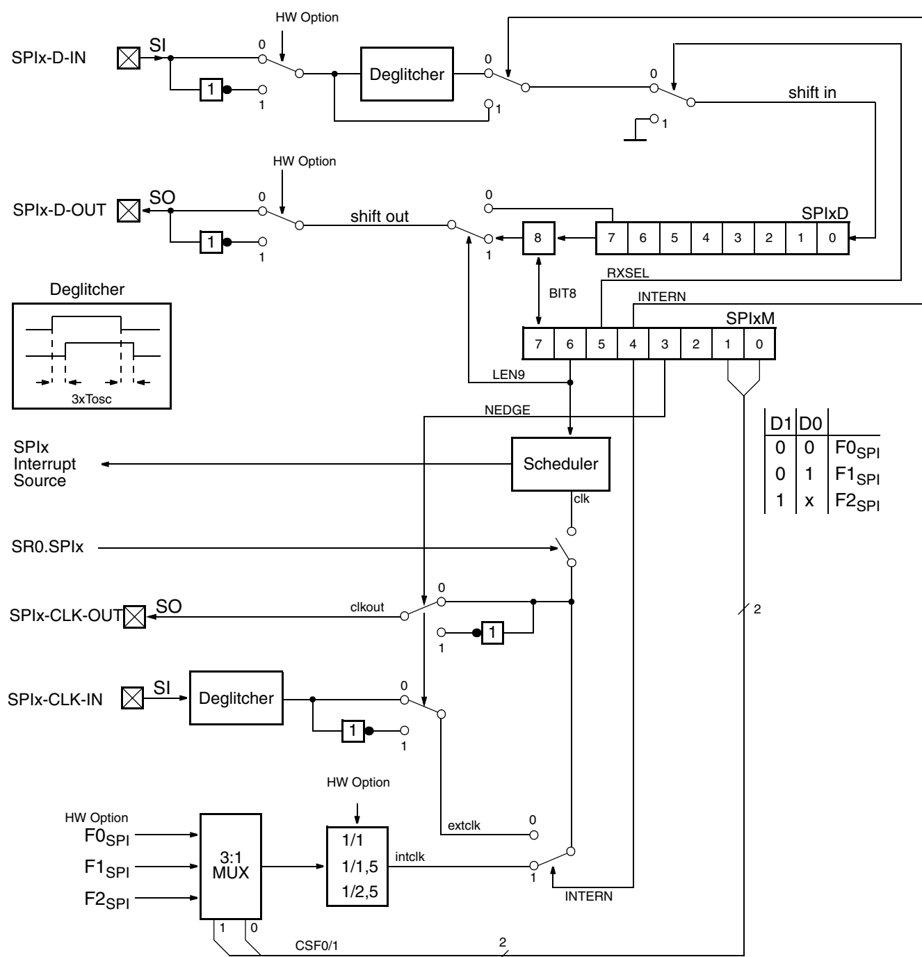
Fig. 19–1: Block Diagram
