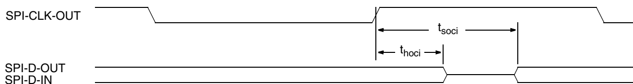
Fig. 3–1: SPI: Send and Receive Data with Internal Clock. Timing is valid for inverted clock too (Data valid at positive edge).
