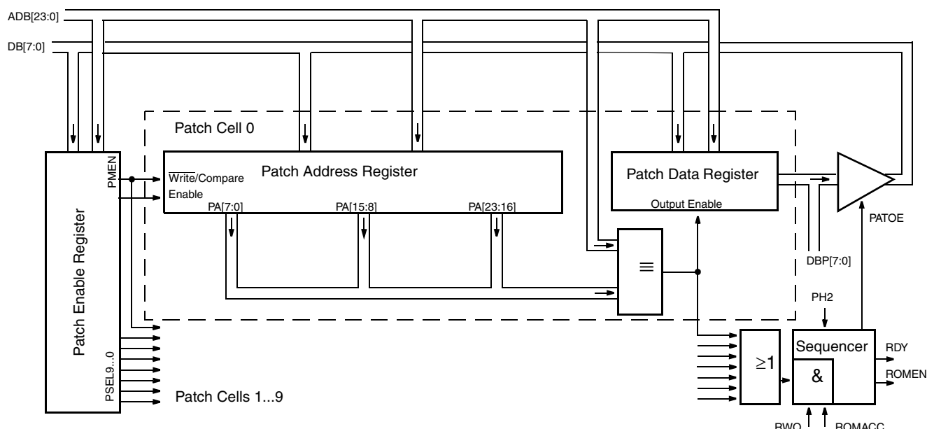
Fig. 9-1: Block Diagram
