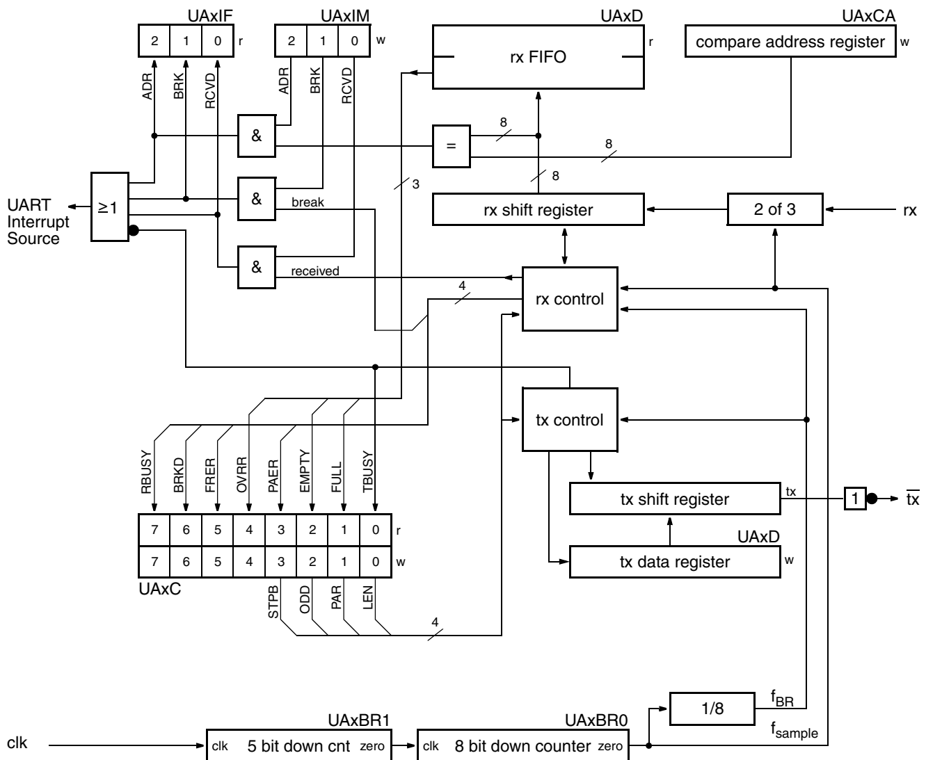
Fig. 20–1: Block Diagram
